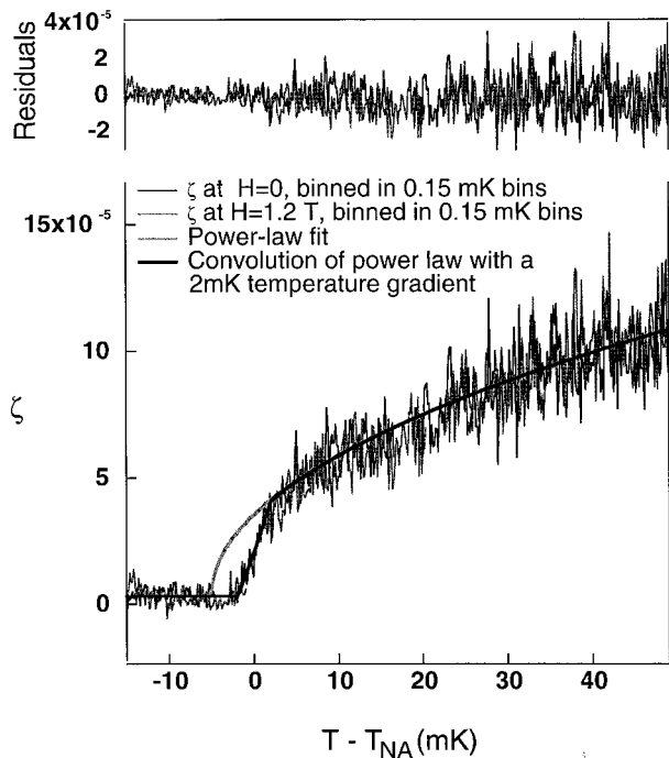
Figure 1. Pure 8CB, d = 30 \mu\text{m} , 0.59 \pm 0.02 \text{ K/cm} . Here t_0 = (5.0 \pm 0.5 \text{ mK})/(307 \text{ K}) = 1.6 \pm 0.1 \times 10^{-5} . Results are shown with and without an external applied magnetic field.
